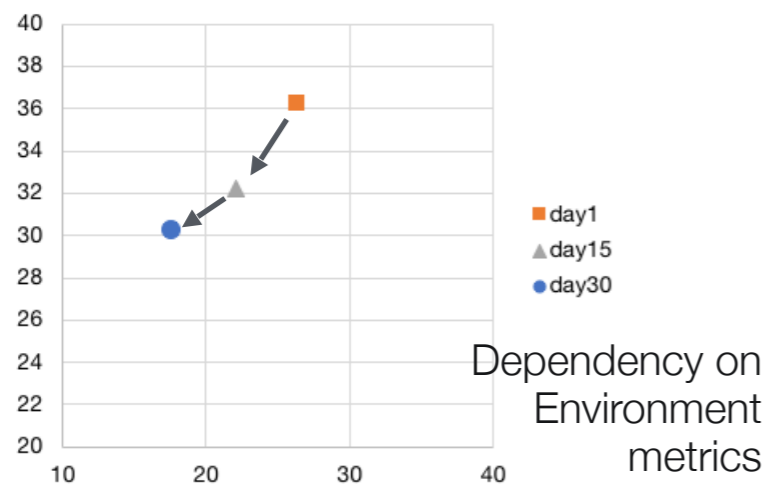
Performance metrics
